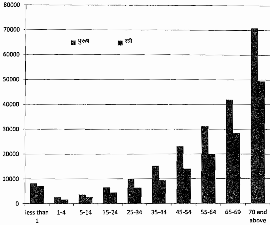
Age-wise sex-wise trends of number of deaths in 2017
